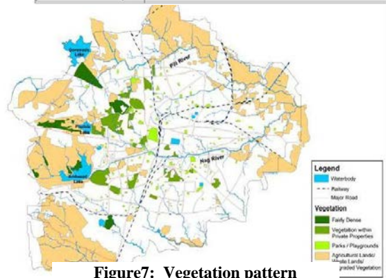
Figure7: Vegetation pattern
